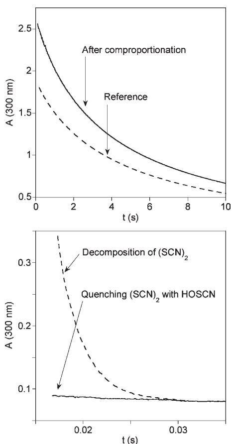
Figure 4. Change in absorbance at 300 nm after directly mixing solutions of (\text{SCN})_2 and HOSCN/OSCN − at pH = 0.70 (top) and at pH = 3.89 (bottom). At pH = 0.70, HOSCN comproportionates with SCN − to give (\text{SCN})_2 which decomposes in a homogeneous second-order reaction. [(\text{SCN})_2]_{\text{T},0} = 1.4 \text{ mM} , [\text{HOSCN}]_{\text{T},0} = 1.1 \text{ mM} , [\text{SCN}^-] = 0.25 \text{ M} , [\text{HClO}_4] = 0.20 \text{ M} , \mu = 1.0 \text{ M} , and 25.0 \text{ }^\circ\text{C} : (dashed line) reference ( [\text{HOSCN}]_{\text{T},0} = 0 ); (continuous line) experiment. At pH = 3.89, HOSCN/OSCN − quenches (\text{SCN})_2 . [(\text{SCN})_2]_{\text{T},0} = 1.4 \text{ mM} , [\text{HOSCN}]_{\text{T},0} = 1.2 \text{ mM} , [\text{SCN}^-] = 0.25 \text{ M} , [\text{HOAc}] + [\text{OAc}^-] = 0.50 \text{ M} , \mu = 1.0 \text{ M} , and 25.0 \text{ }^\circ\text{C} : (dashed line) reference ( [\text{HOSCN}]_{\text{T},0} = 0 ); (continuous line) experiment.
